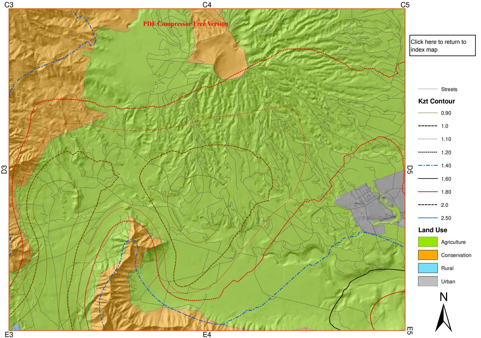
Wind Topographic Factor (Kzt) for the Island of Kauai (D4)
