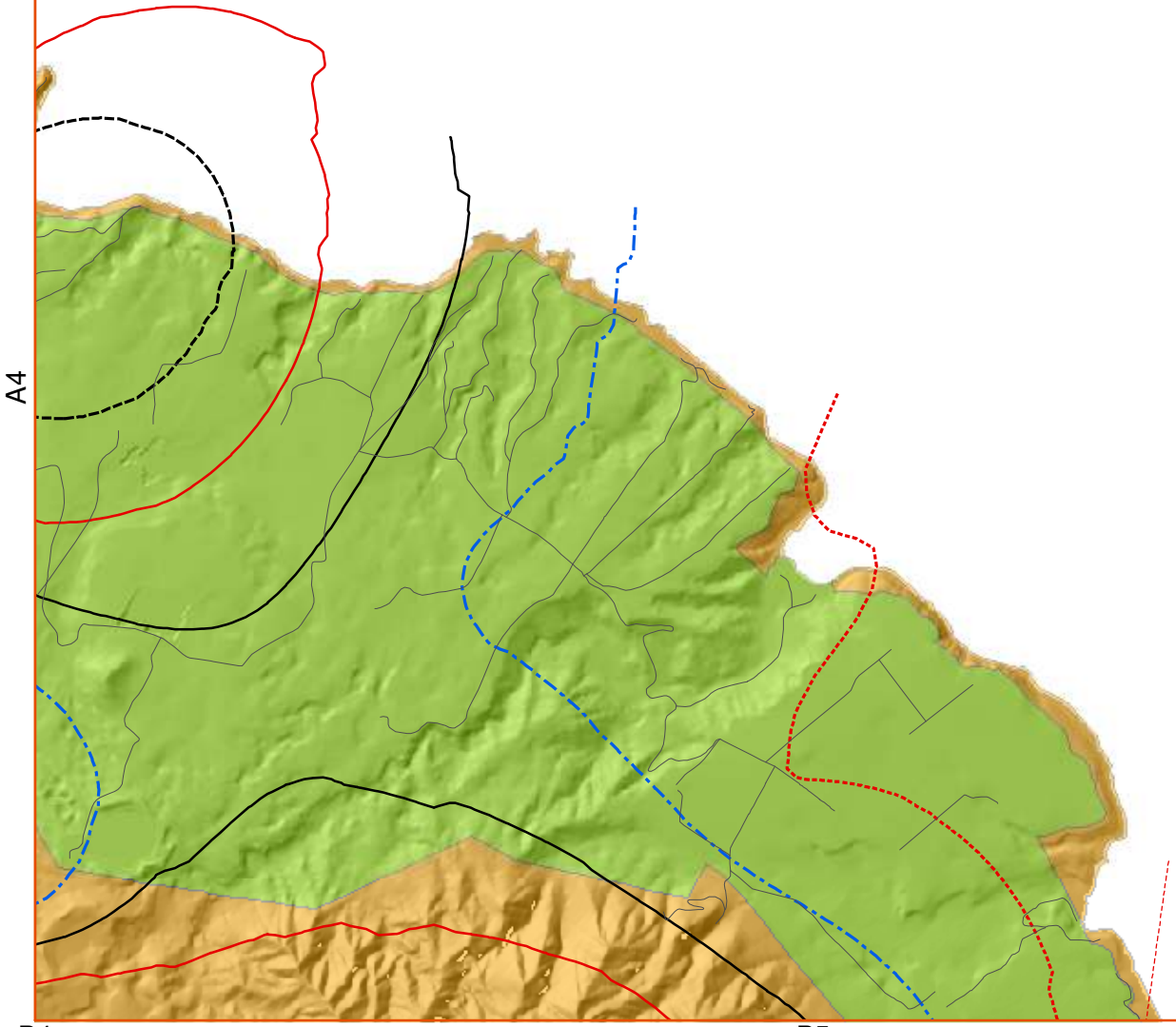
Wind Topographic Factor (Kzt) for the Island of Kauai (A5)
