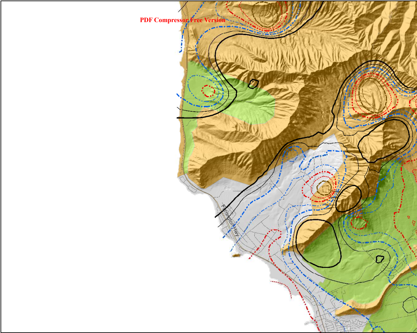
Kzt Contour for the Island of Oahu (C1)
